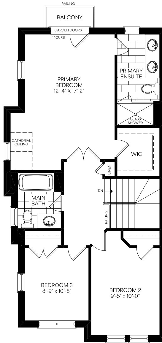
Third Floor Optional 4 PC Ensuite Elevation B1
