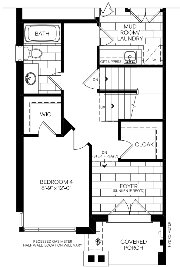
Ground Floor Optional 4 Bedroom Plan Elevation C
