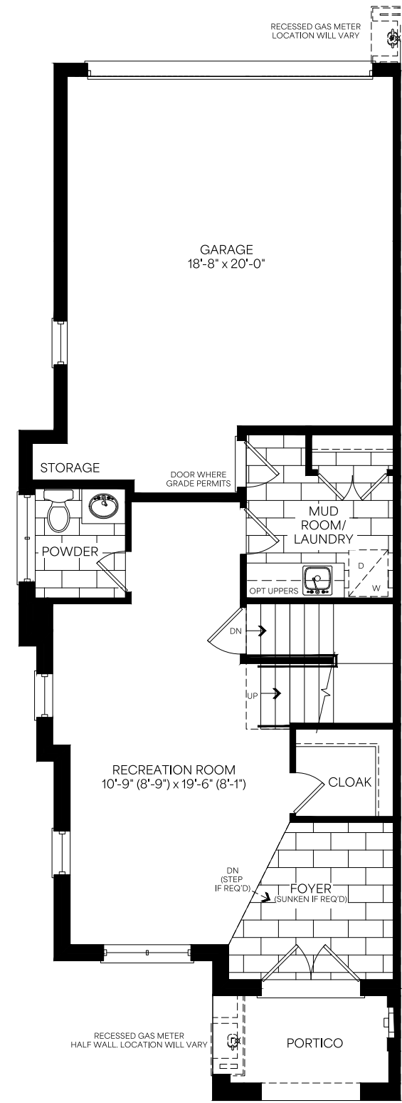
Ground Floor Elevation B1
