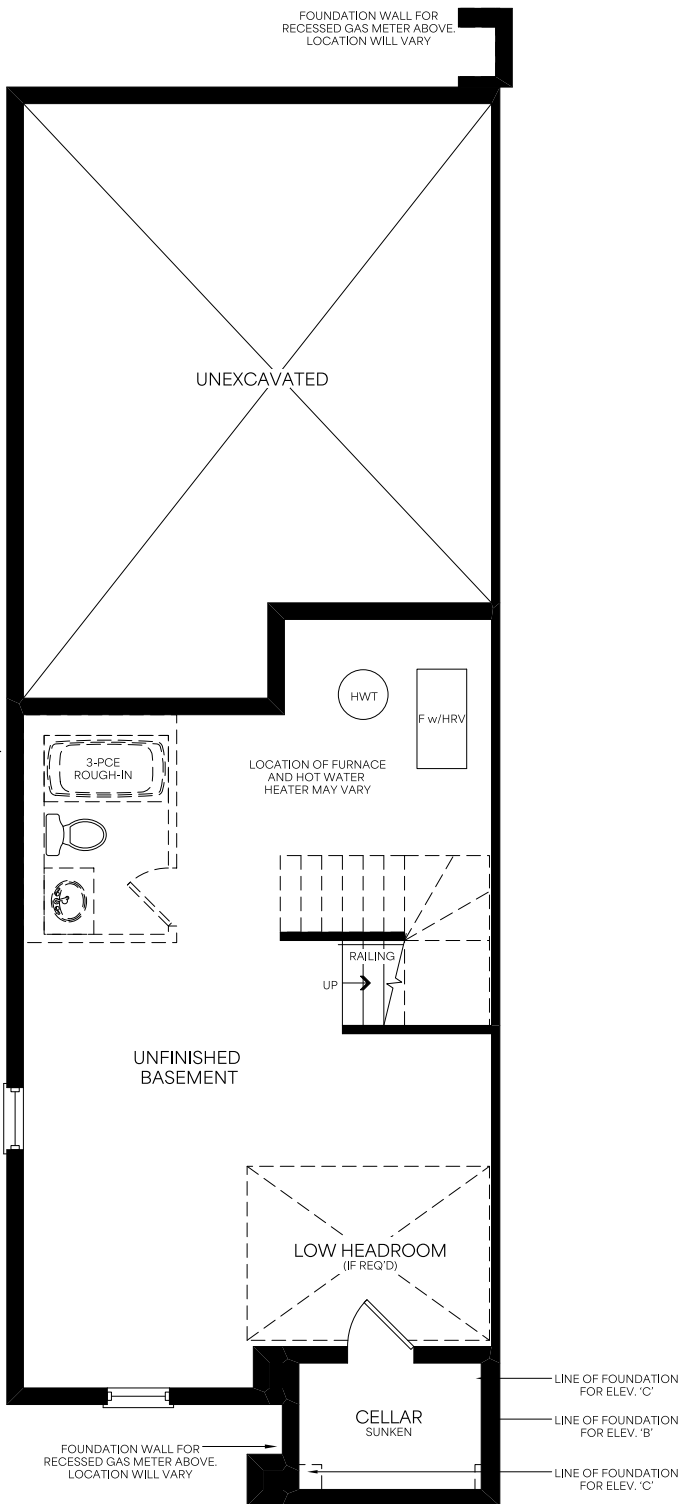
Basement Elevation C
