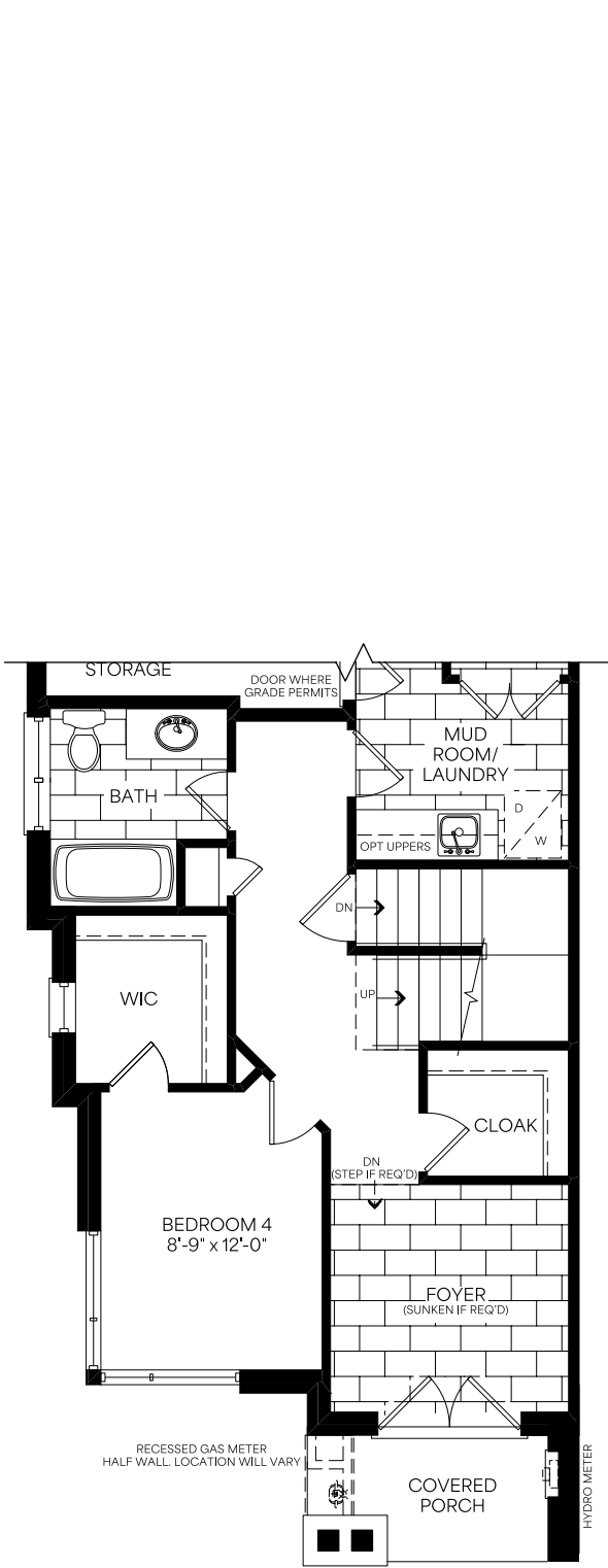
Ground Floor Optional 4 Bedroom Plan Elevation C
