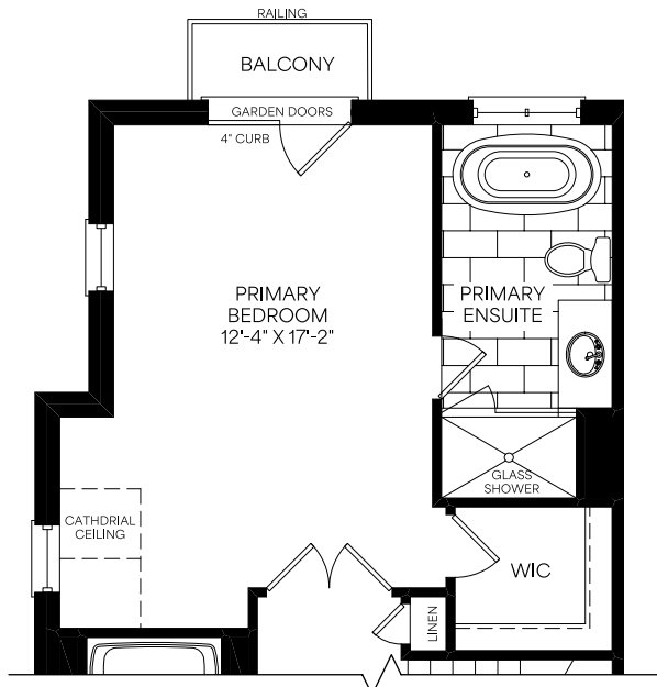
Third Floor Optional 4 PC Ensuite Elevation B1
