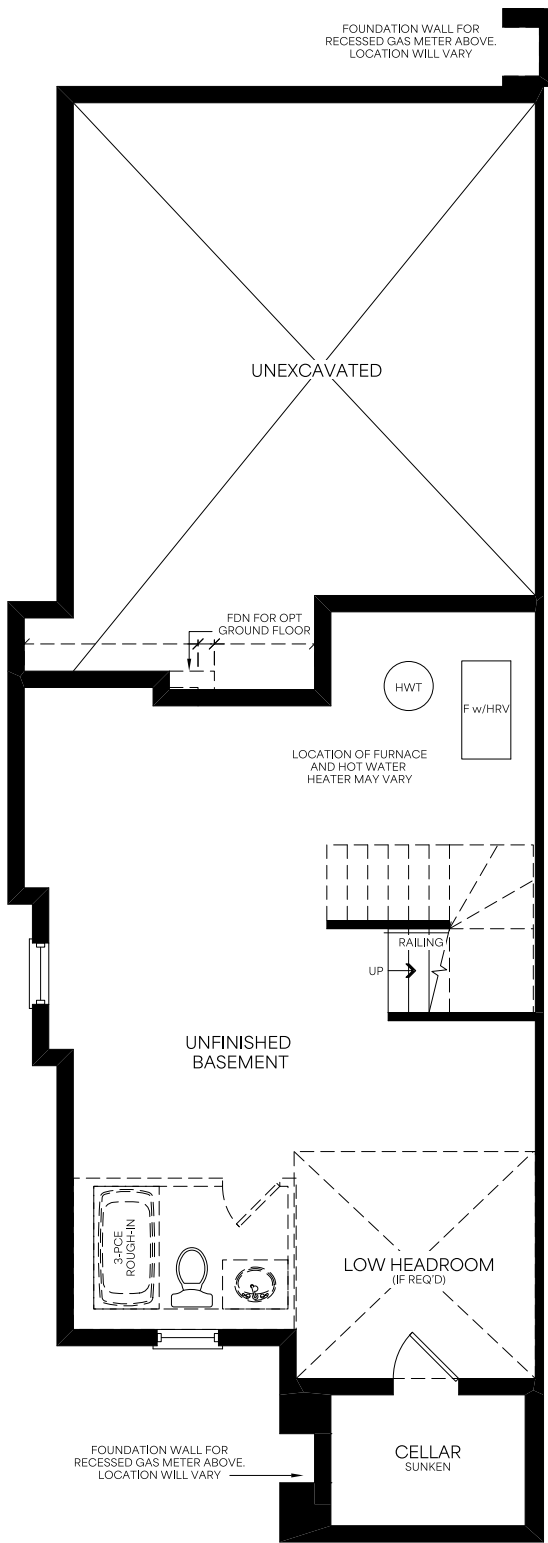
Basement Elevation B1
